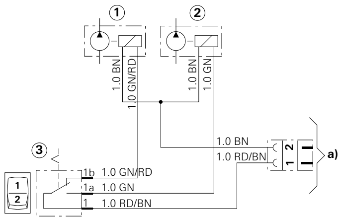
Changeover switch without cover
